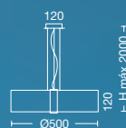
ART: CT28050 Color: Cromado 3xE27 LED
